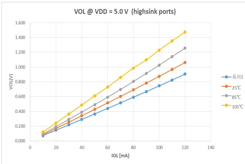
Figure 3-3 VOL(highsink ports) 温度曲线
