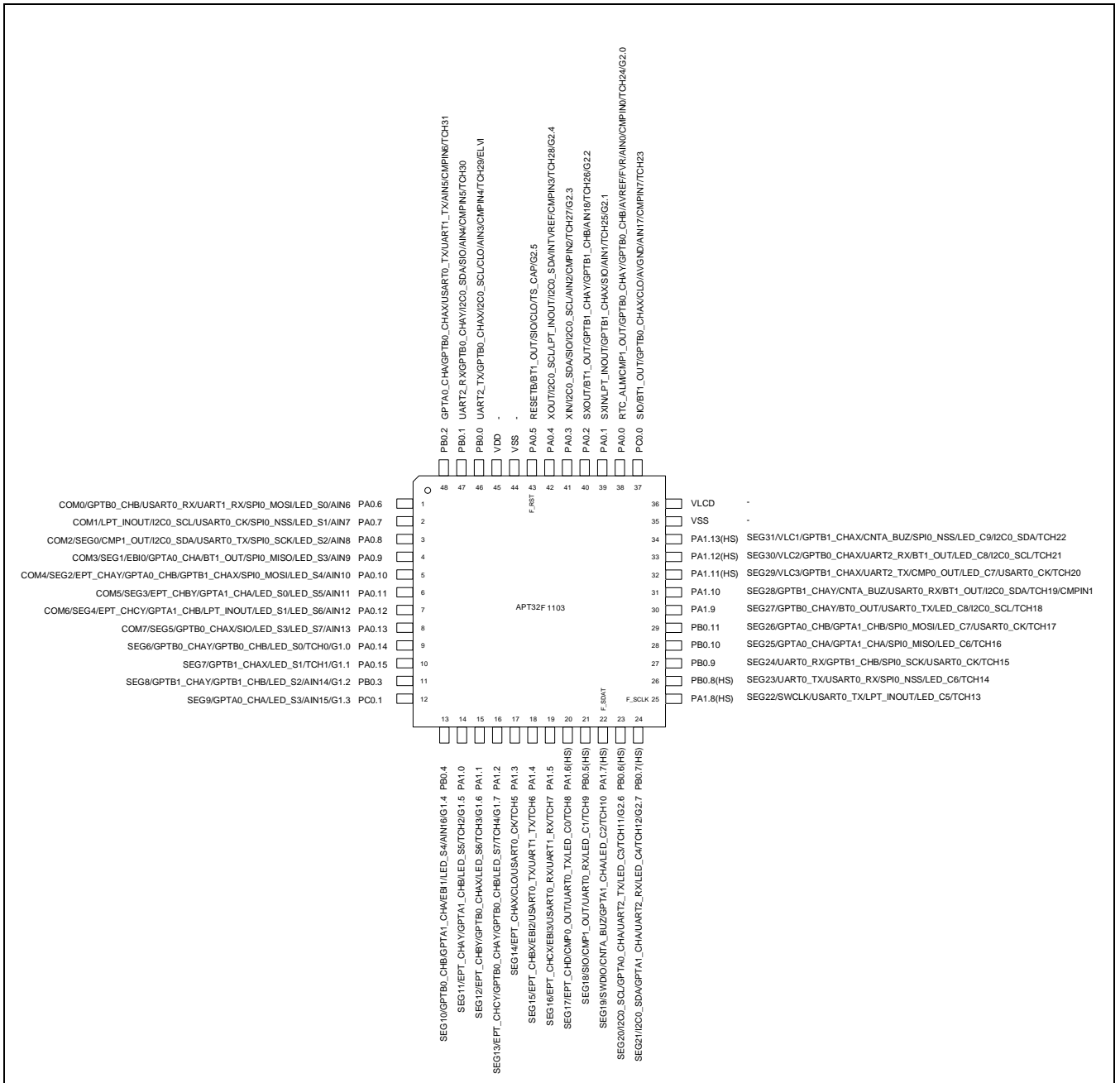
Figure 2-1 管脚定义图(48 LQFP/QFN)
