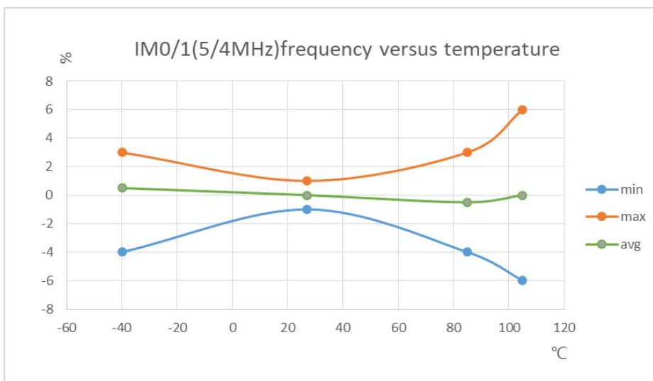
Figure 3-7 IM_5/4M频率温度曲线
