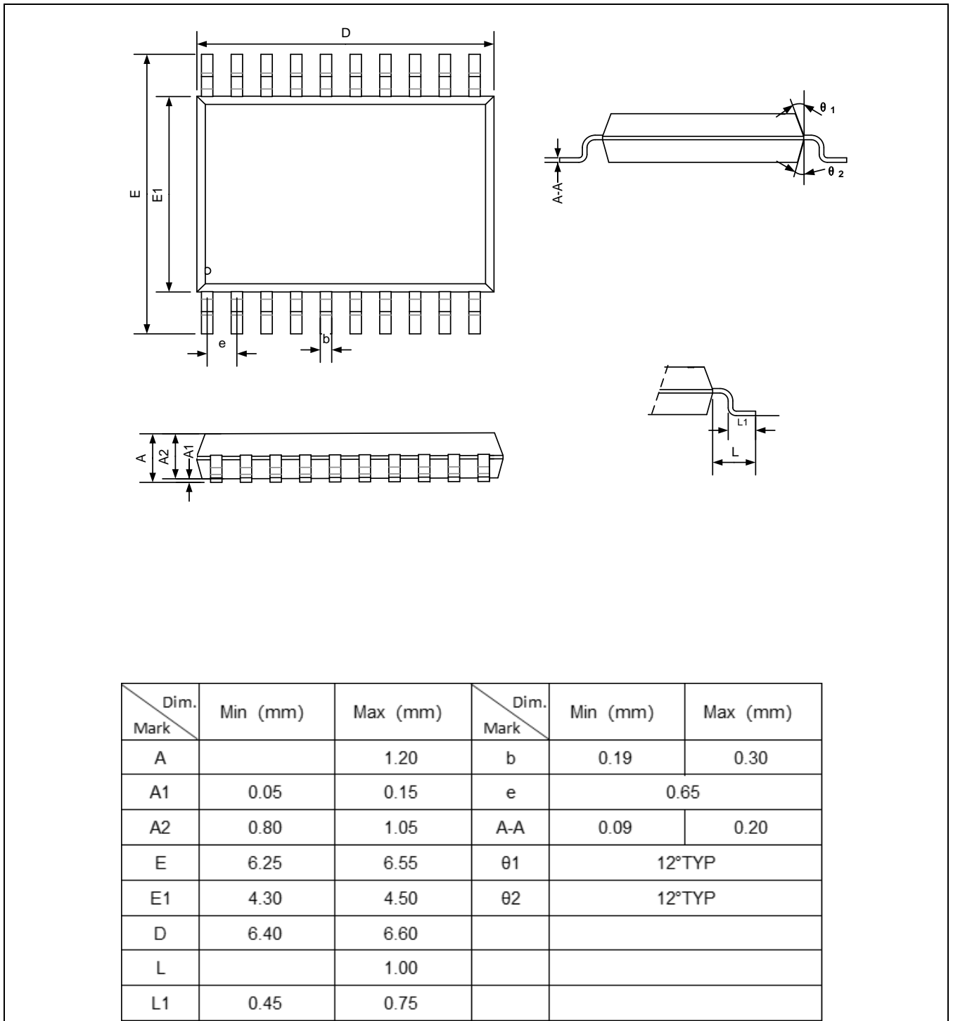
Figure 4-1 TSSOP20 (0.635mm)封装尺寸
