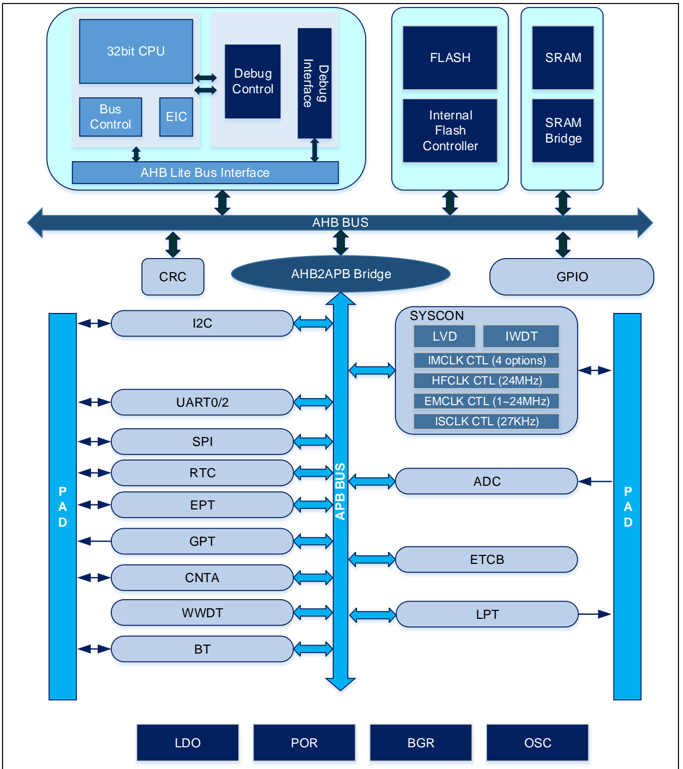
Figure 1-1 APT32S003BF7P6模块框图
