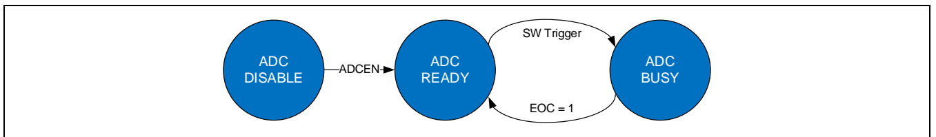
Figure 9-3 ADC状态机
